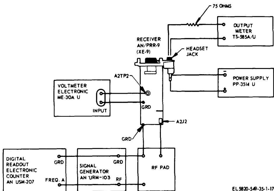
Figure 4-8. AN/PRR-S(XE-9) if. selectivity test.
